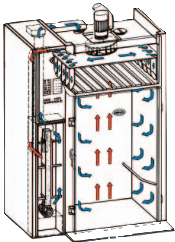
Schematic diagram of the CIRCO-SYSTEM ®
